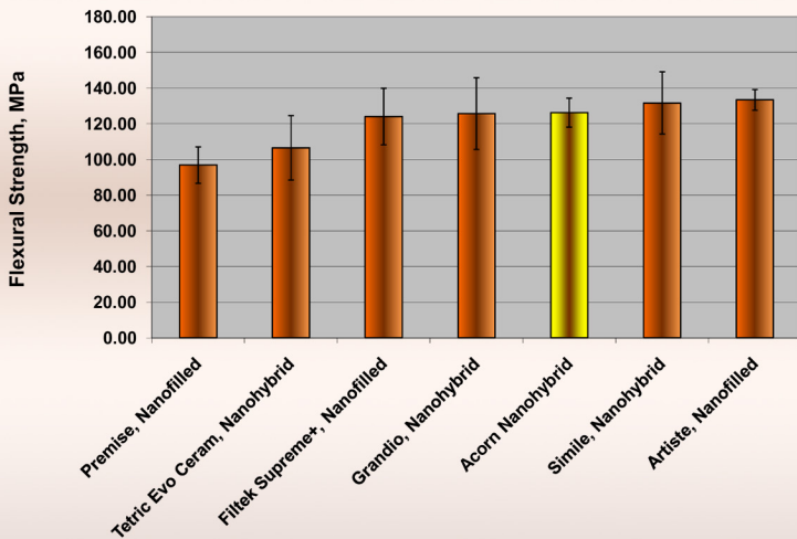
Flexural Strength
